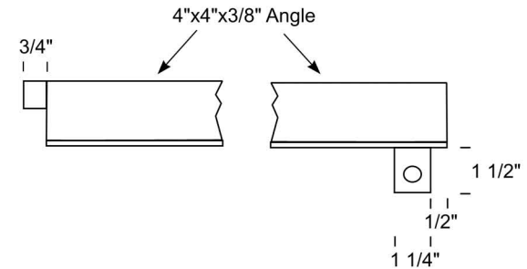
Sectional View Bat Guards Removed For Clarity
