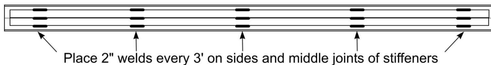
Horizontal Bar Design with Stiffener
